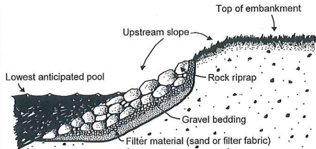
Figure 2 - Rock Riprap
