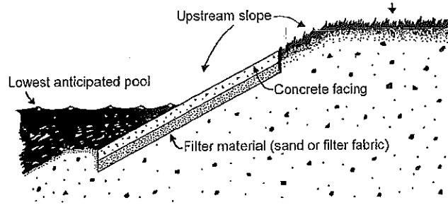
Figure 4 - Concrete facing
