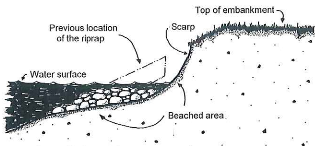
Figure 1 - Beaching
